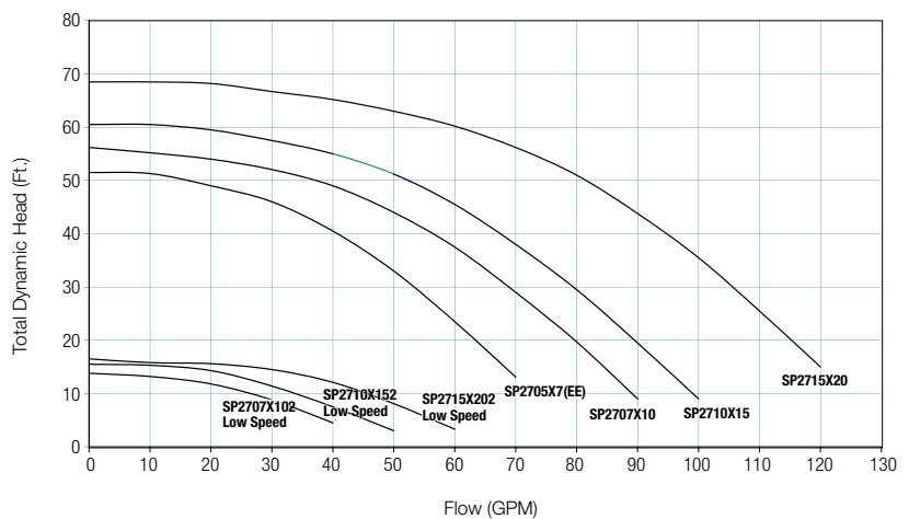
Performance Curves – Max-Flo II (Improved) Pump
